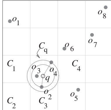
Query Processing – k NN, Fig. 1 Grid-based k NN computation
