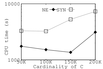
Figure 4: Scalability for large data
