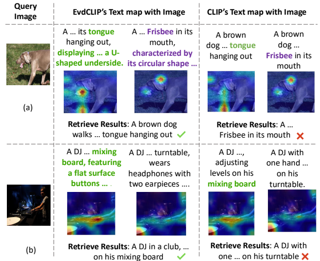
Figure 4: Visualization examples of retrieval. We present image queries (the first column) along with four heatmaps.
