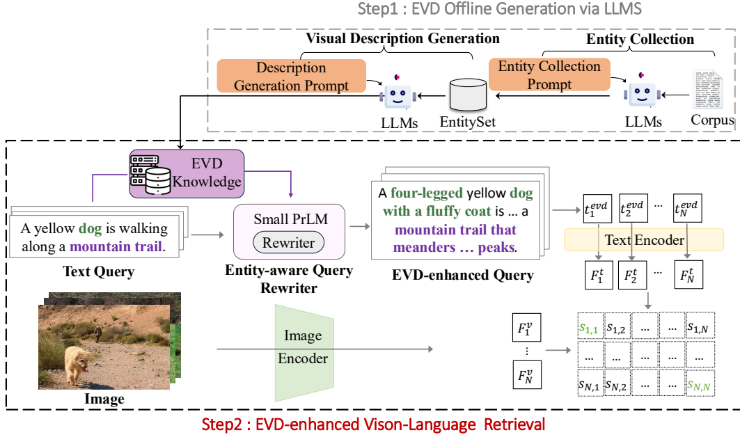
Figure 3: The overall architecture of EvidCLIP comprises two components: EVD offline generation via LLMs and EVD-enhanced vision-language retrieval. First, EVD knowledge is generated offline using LLMs. Then, an EVD-aware query rewriter integrates the query with EVD to produce an EVD-enhanced query for retrieval.
