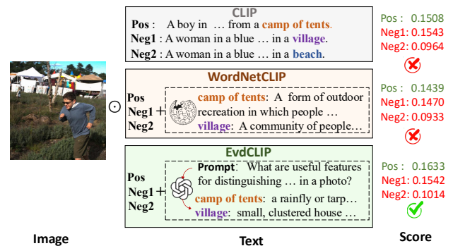
Figure 1: Illustration of entity visual descriptions (EVD) enhanced framework. The CLIP and WordNetCLIP which introduces the concept of entities struggle to distinguish between “camping of tents” and “village”, leading to incorrect retrieval results. Our EvdCLIP leverages the EVD generated by LLMs to improve cross-modal retrieval performance.
